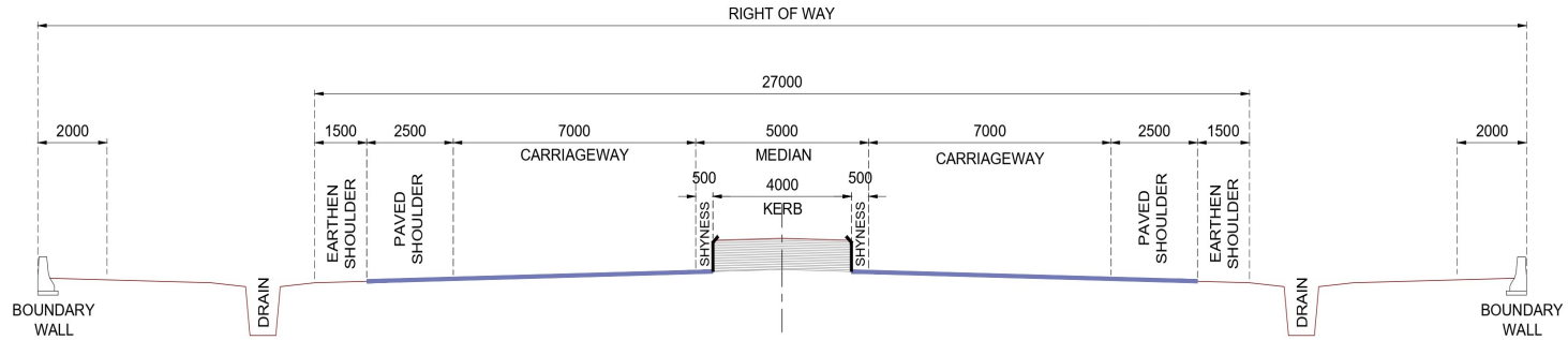
TYPICAL CROSS SECTION (4 LANE HIGHWAY WITHOUT SERVICE ROAD AND WITH RAISED MEDIAN)
