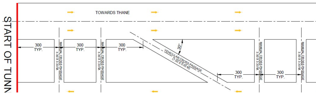
Typical details of Pedestrian Cross passage spacing at 300m and vehicular cross passage after every two pedestrian cross passages
