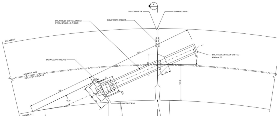
Figure 15: Typical View of the Radial Joint in a Segmental Lining
