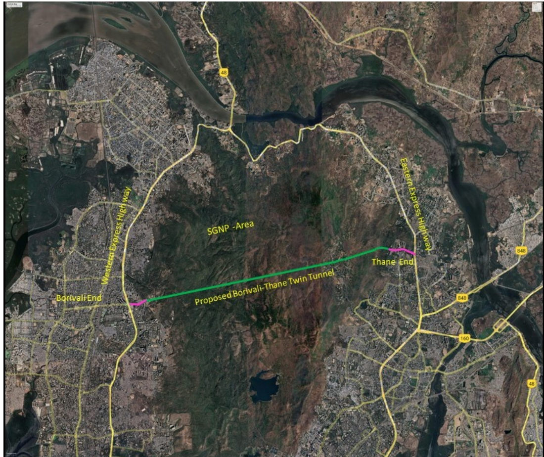
Fig. 4-1 Alignment of Proposed Thane-Borivali Tunnel
