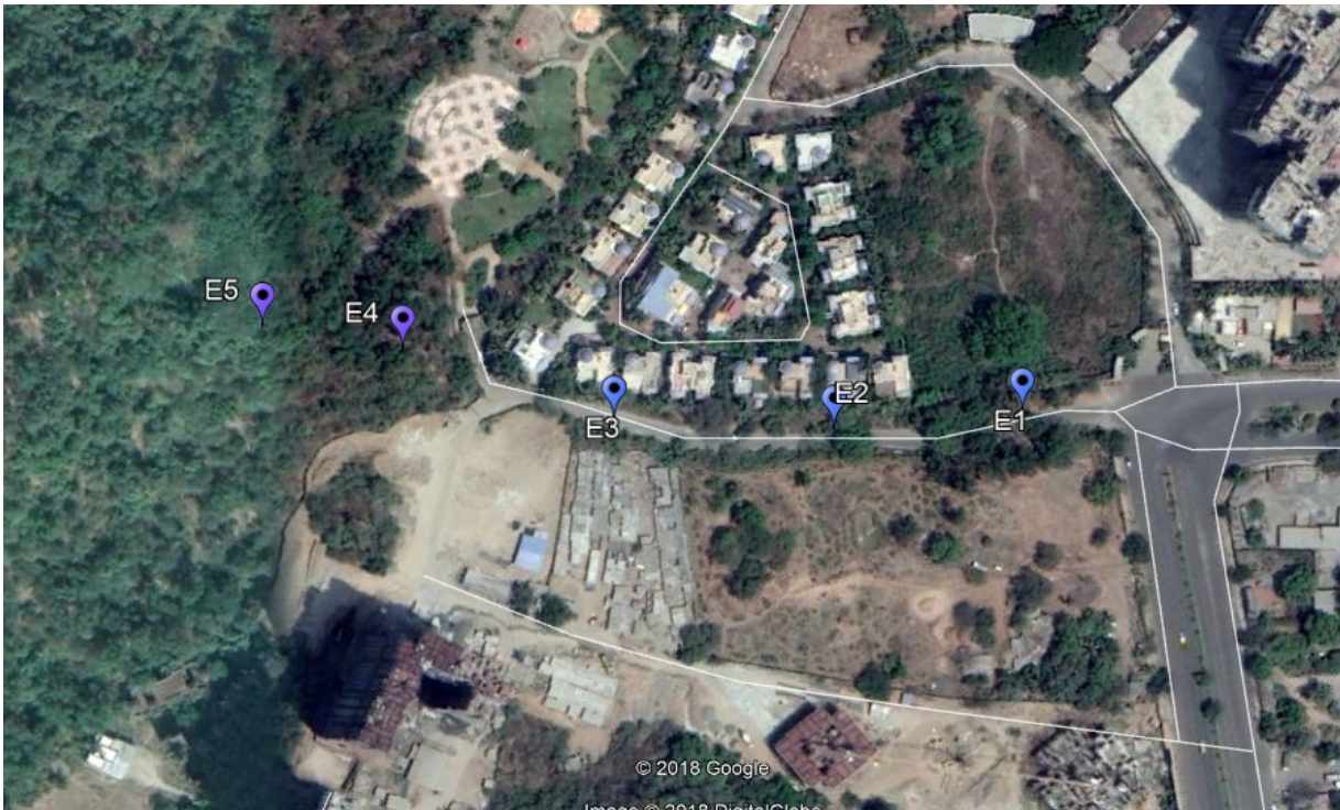
Figure 5.16: Location Plan for Boreholes near Eastern portal
