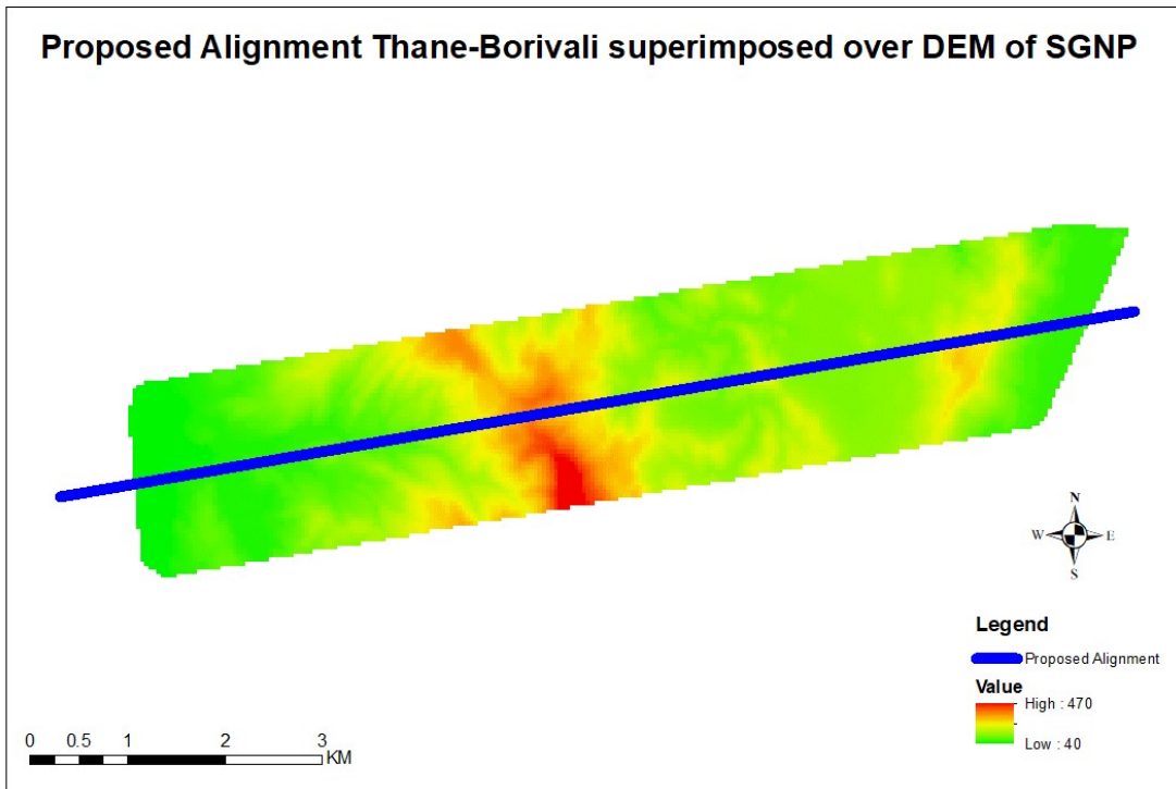
Figure 5.1: Proposed TBHT alignment with DEM inside SGNP
