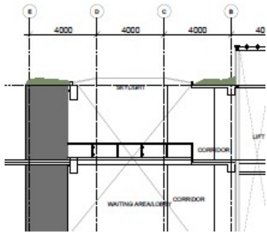
Typical section of Control centre building
